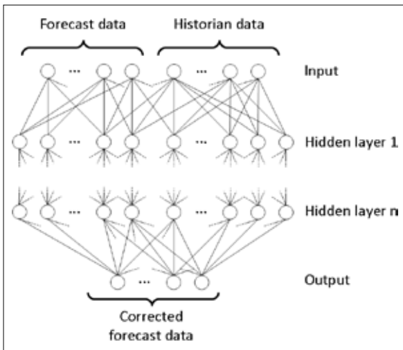
Figure 2: Neural network to tailor the model
