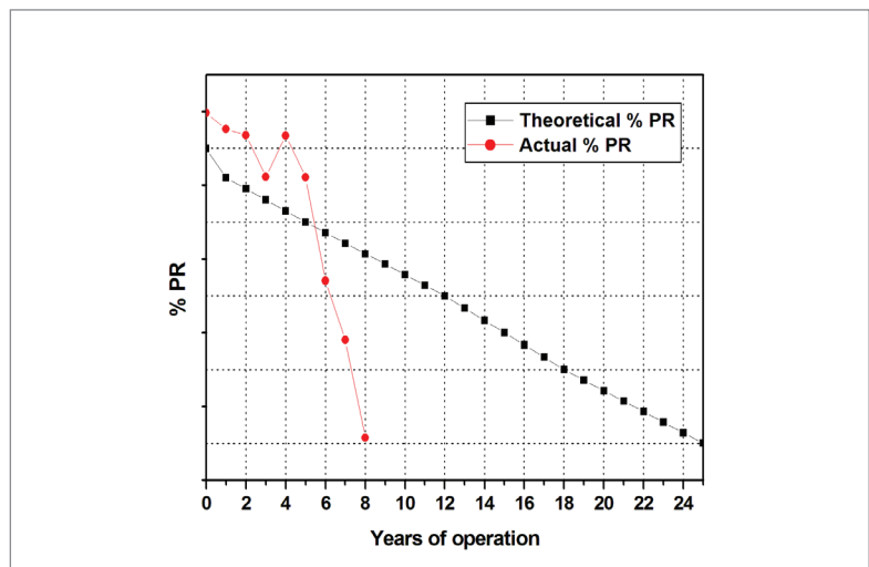
Figure 6. Actual PR degradation case installed in Southeast Asia.
