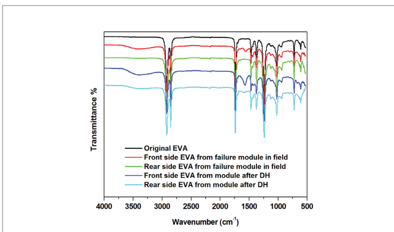
Figure 8. FTIR spectra of EVA from modules in field and after DH.
